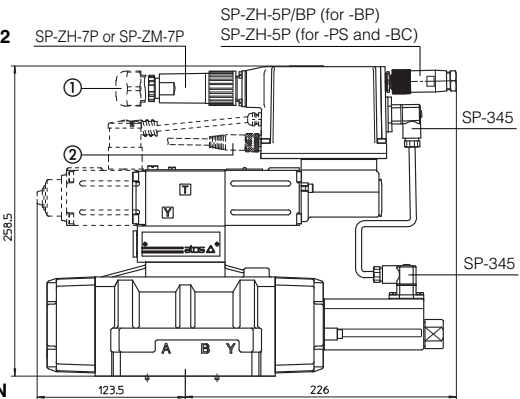
DPZO-TES*-2
