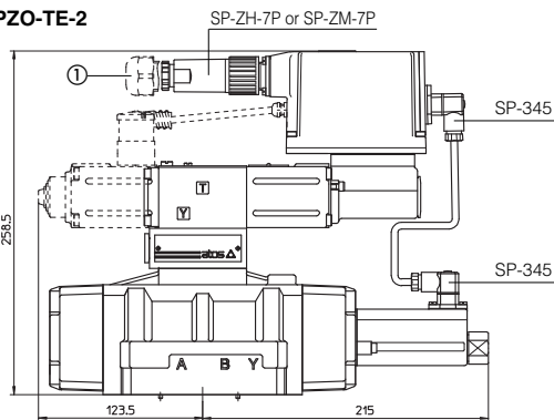
DPZO-TE-2
